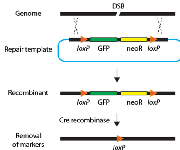
Figure 4. Diagram of streamlined CRISPR-Cas. The streamlined strategies integrate a drug-resistance gene (yellow), a fluorescence marker (green), and a Cre recombinase to facilitate smooth genome editing by removing these two markers.
