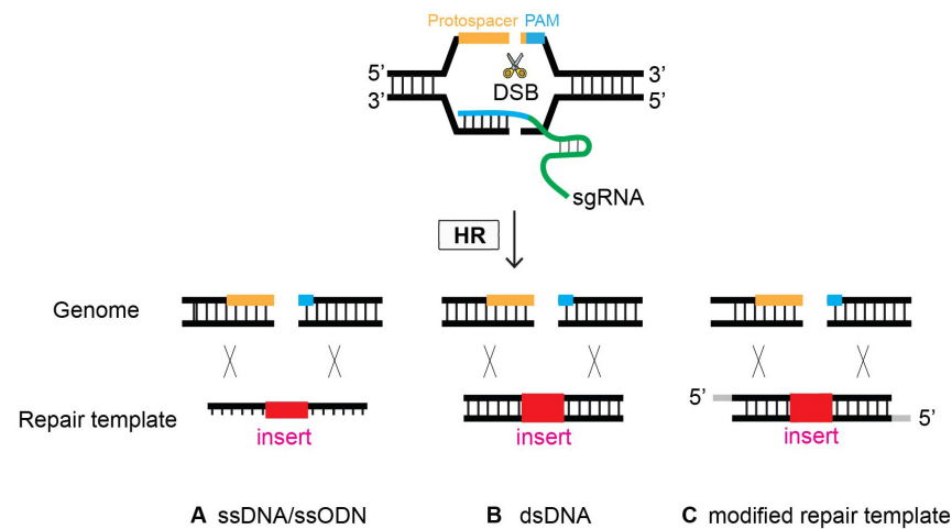
Figure 7. Oligonucleotides can serve as a template to repair DSBs via HR. At the site of CRISPR-Cas9-induced DSB, Single-stranded DNA (ssDNA), double-stranded DNA (dsDNA), and modified repair templates serve as a repair template. (A) ssDNA, (B) dsDNA, and (C) modified nucleotides as a repair template.
