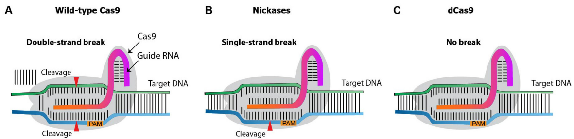
Figure 5. Diagram illustrating different types of Cas9 variants. (A), wild-type Cas9 nuclease. (B), Cas9 nickases that introduce a single-strand break at the target DNA. (C), catalytically inactive (dead) dCas9, which induces no breaks.
