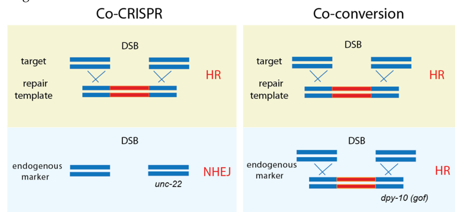
Figure 3. Co-CRISPR and co-conversion. Both methods employ an endogenous marker gene that exhibits phenotypic changes, thus ensuring that proper genome editing is processed. While Co-CRISPR uses NHEJ for targeting marker genes, co-conversion relies on homologous recombination (HR) via a repair template.
