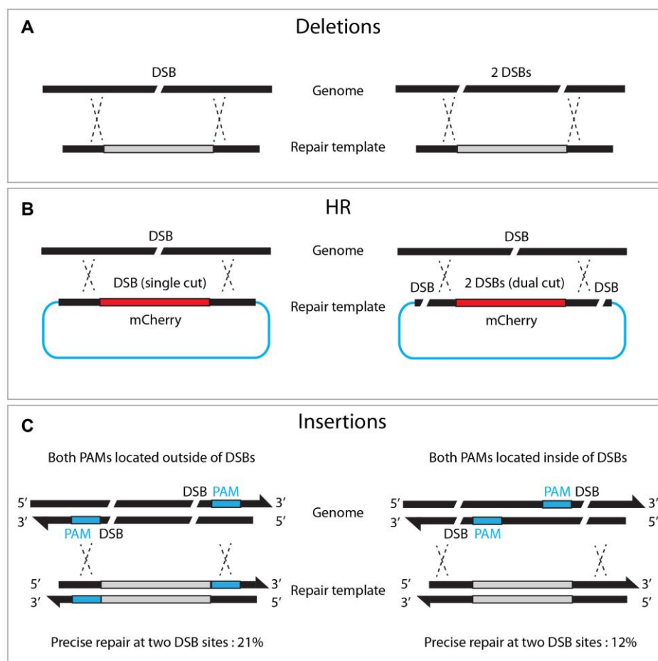
Figure 6. Dual DSBs enhance deletions, homologous recombination, and insertions. (A) Single versus dual DSBs at targeted sites. (B) Dual DSBs (right) in the repair template enhances HR efficacy compared to single DSB (left). (C) Locating both PAMs outward of the DSB sites enhances insertion frequency.
